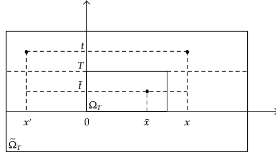
Figure 1: Case (x, t), (x', t) \in \tilde{\Omega}_T with \bar{x} = \bar{x}' .
