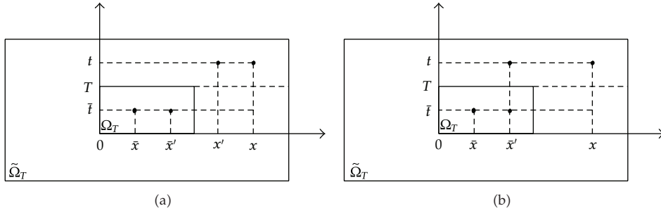
Figure 2: Case (x, t), (x', t) \in \tilde{\Omega}_T with \bar{x} \neq \bar{x}' . (a): x' \neq \bar{x}' . (b): x' = \bar{x}' .
