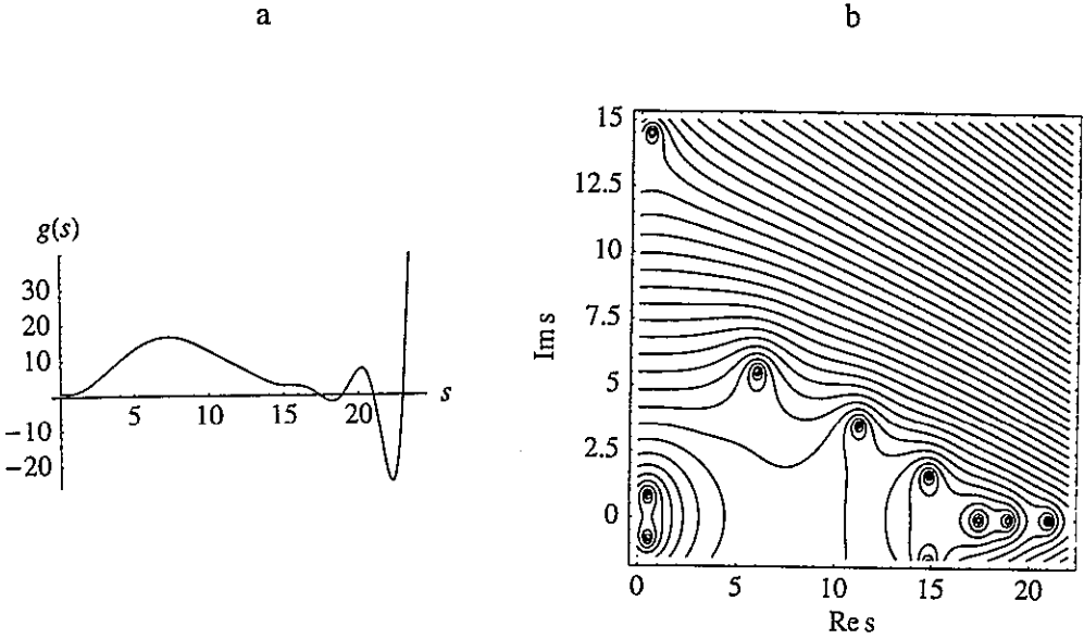
Figure 3. The function g(s) , whose zeros are the same as the first term of the Riemann-Siegel main sum, (a) on the real s axis, (b) contours of |lg(s)| , showing zeros enclosed by loops.
