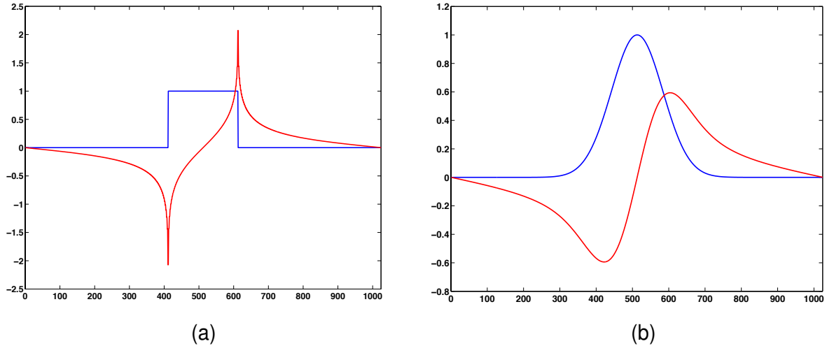
Fig. 1. Scaling functions and their Hilbert transforms: (a) The discontinuous Haar scaling function (BLUE) and its transform (RED), (b) The smooth cubic B-spline (BLUE) and its transform (RED). In either case, the transformed function is “broken-up” and, as a consequence, loses its approximation property. In particular, the transform no longer exhibits the partition-of-unity property, which is characteristic of scaling functions. Also, note the slow decay of the transform, particular for the smooth spline function. In fact, both the transforms decay as 1/|x| —the smoothness of the original function has no effect on the decay of the transform.
