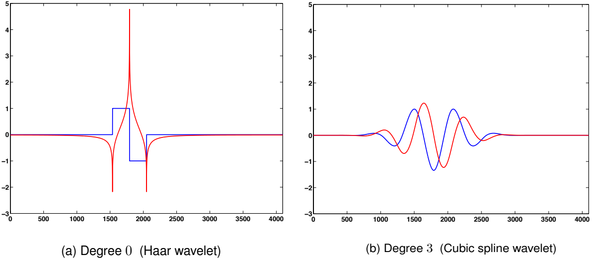
Fig. 3. B-spline wavelets (shown in BLUE) and their Hilbert transforms (shown in RED). The wavelets are ordered (left to right) by increasing smoothness and vanishing moments; both are compactly supported. Notice how the decay of the Hilbert transform increases with the increase in vanishing moments—the transform of the cubic spline wavelet appears to have an almost identical localization. Moreover, it is as smooth as the original wavelet. It is shown in the text that, in the presence of some minimal smoothness, the Hilbert transform is as smooth and oscillating as the spline wavelet.
